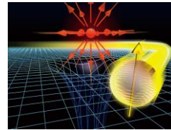
Berry phase emerging from spin-ice state
